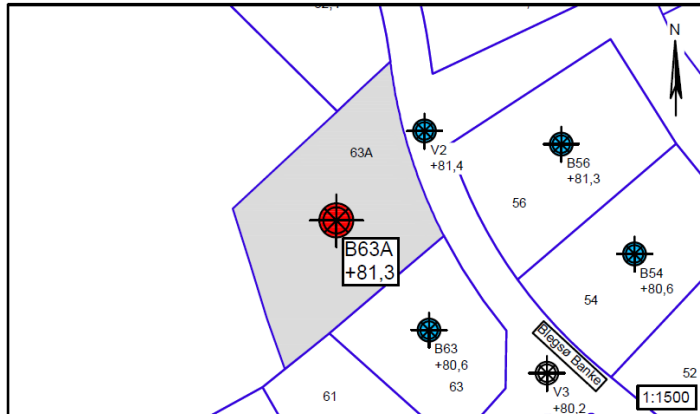
Figur 1 – Situationsplan 1:1500, Parcel nr. 63A
