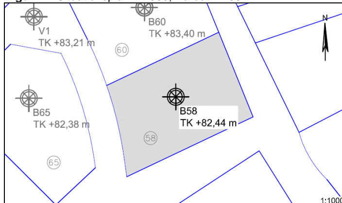
Figur 1 – Situationsplan 1:1000, Parcel nr. 58
