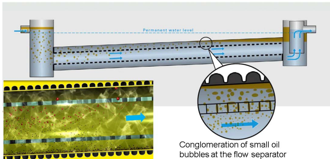
Figure 1.3: Gravity and coalescence principle. Separation of light liquids with SediPipe
